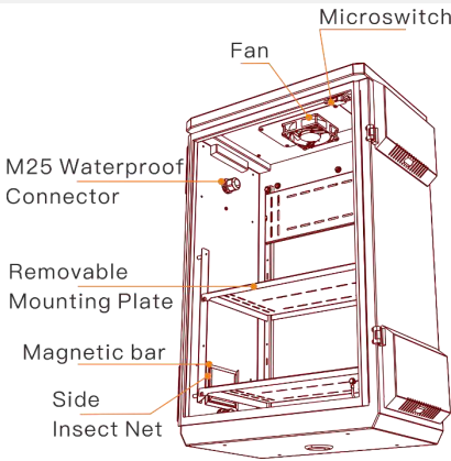
Inner Front
