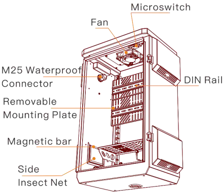
Inner Front
